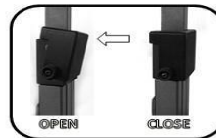
3 Lift up till the bed reaches its upper lock position. A clicking noise on both sides inform that the safety devices are activated. Make sure about it, otherwise do it manually by moving the safety devices into the closed position.
