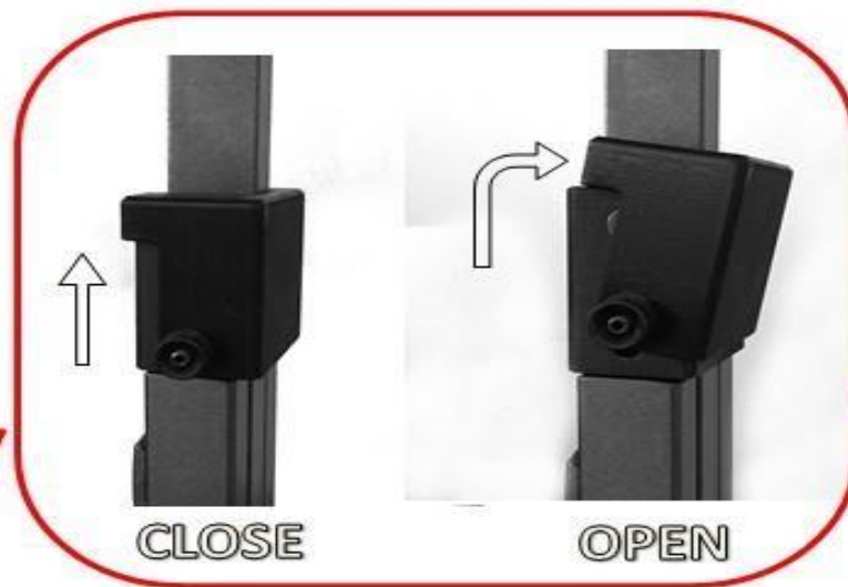
5 Unlock the left safety device by moving it up and forwards keeping it in a tilted position
